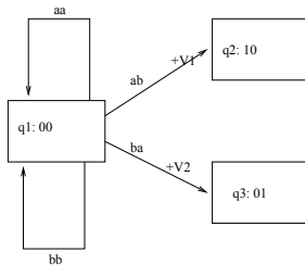
Figure 1: Simple AATS
