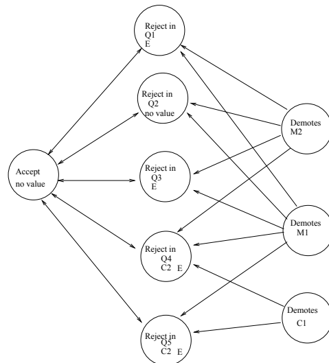
Figure 2: VAF for acceptance or rejection
