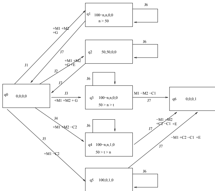
Figure 2: AATS for Ultimatum Game
